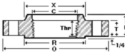
Threaded Flange
