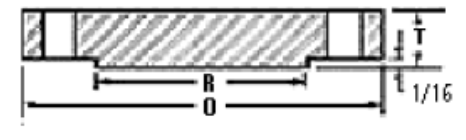
Blind Flange
